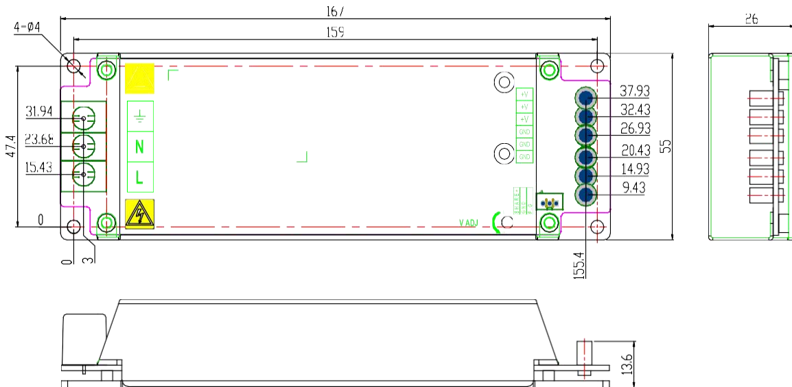
Dimensions and mounting holes - terminal coordinates
